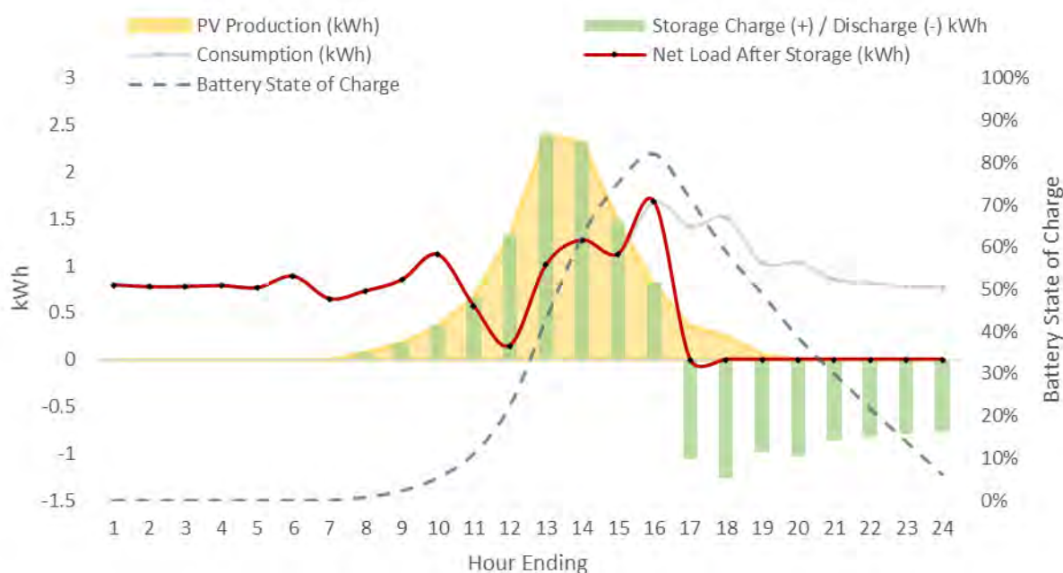
FIGURE 4-3: ILLUSTRATIVE EXAMPLE OF STORAGE DISPATCH, PV SELF-CONSUMPTION
