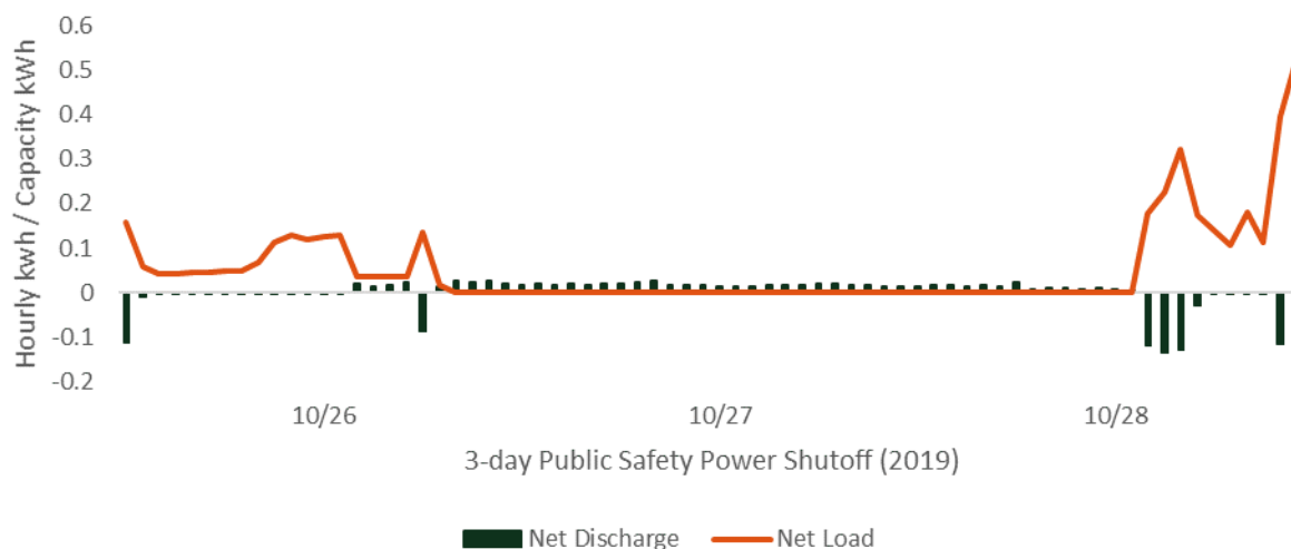
FIGURE 4-60: OBSERVED RESIDENTIAL STORAGE BEHAVIOR DURING PSPS EVENTS (W/OUT SOLAR PV)
