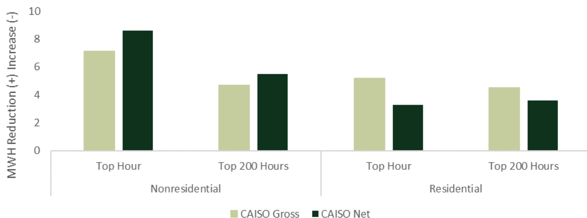
FIGURE 1-7: OBSERVED NET DISCHARGE (MWH) DURING CAISO SYSTEM PEAK HOURS BY CUSTOMER SECTOR
