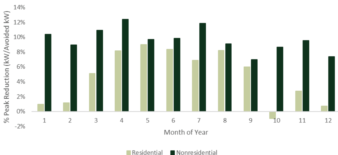
FIGURE 4-18: MONTHLY PEAK DEMAND REDUCTION (KW) PER AVOIDED PEAK (KW)
