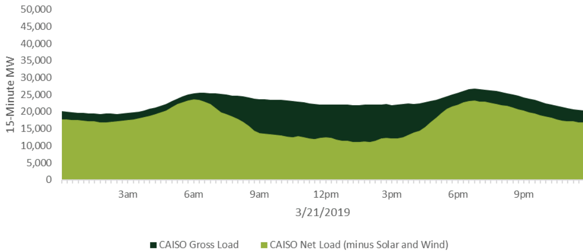
FIGURE 4-34: CAISO NET AND GROSS LOAD ON A TYPICAL EARLY SPRING DAY
