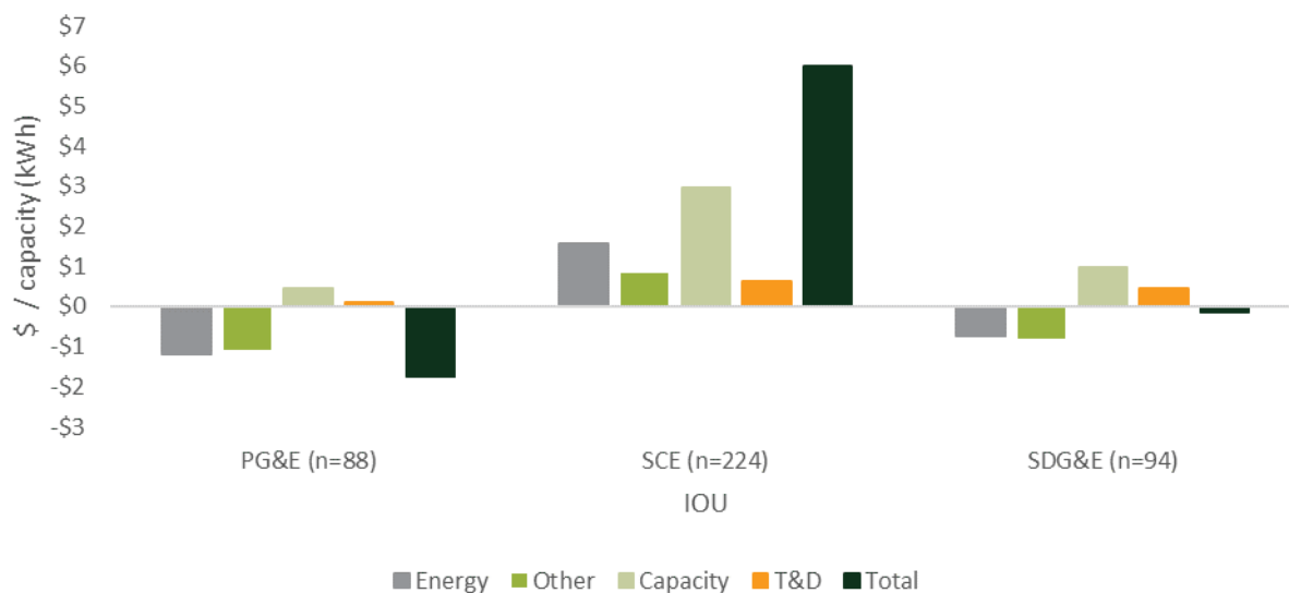
FIGURE 4-55: NONRESIDENTIAL MARGINAL AVOIDED COST $ PER CAPACITY KWH BY IOU
