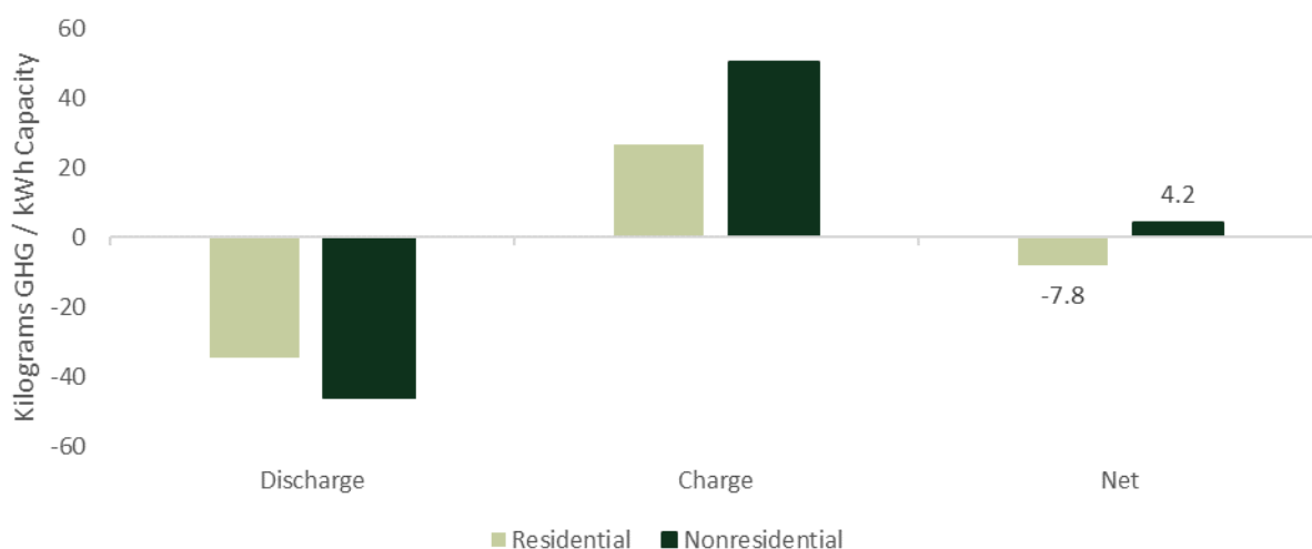
FIGURE 4-47: NET KILOGRAMS CO 2 EMISSIONS PER CAPACITY KWH BY CUSTOMER SECTOR
