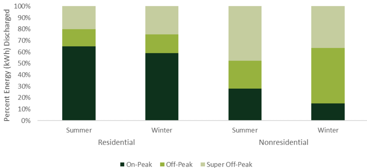
FIGURE 4-10: PERCENT DISCHARGE KWH BY TOU PERIOD AND CUSTOMER SECTOR
