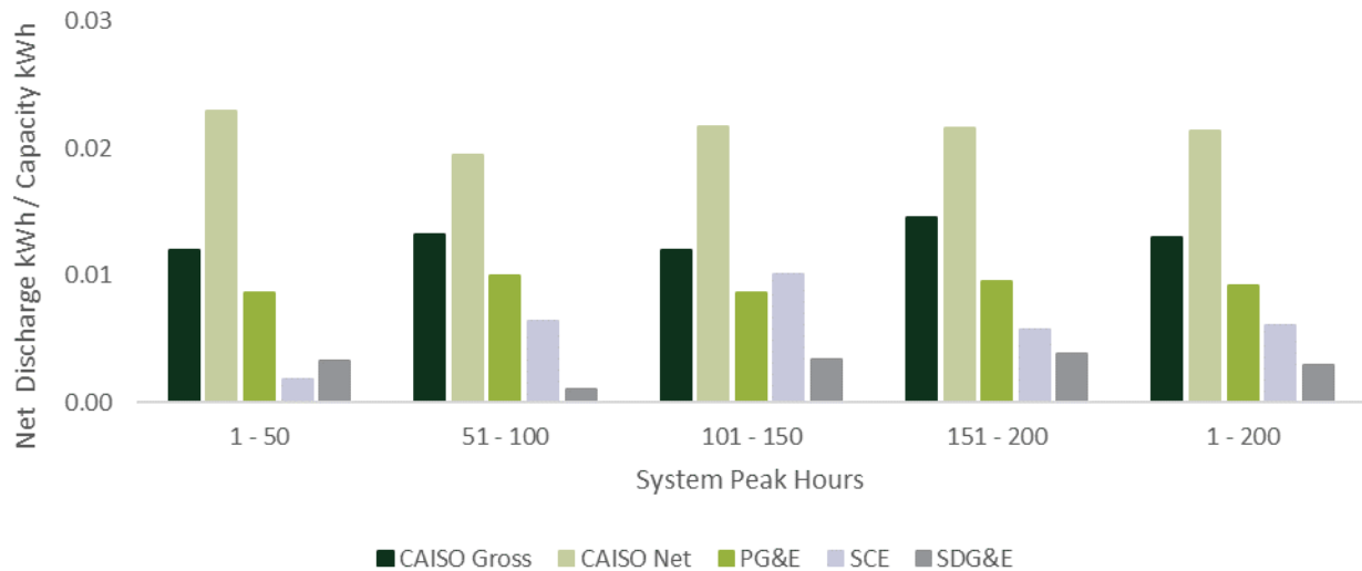
FIGURE 4-43: NET DISCHARGE KWH PER CAPACITY KWH DURING SYSTEM PEAK HOURS FOR NONRESIDENTIAL
