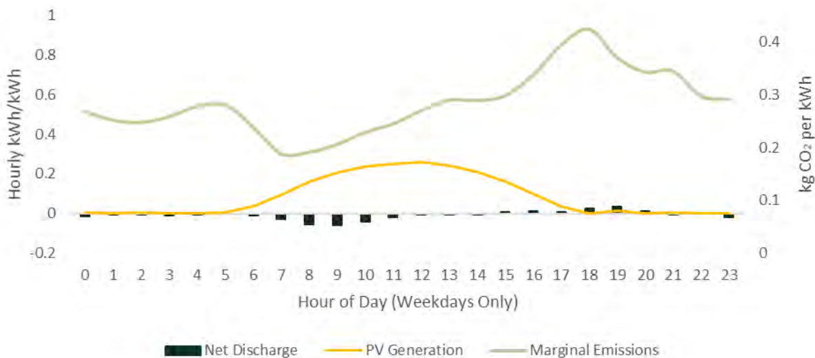
FIGURE 4-54: NONRESIDENTIAL DISCHARGE KWH PER CAPACITY KWH AND MARGINAL EMISSIONS FOR SUMMER
