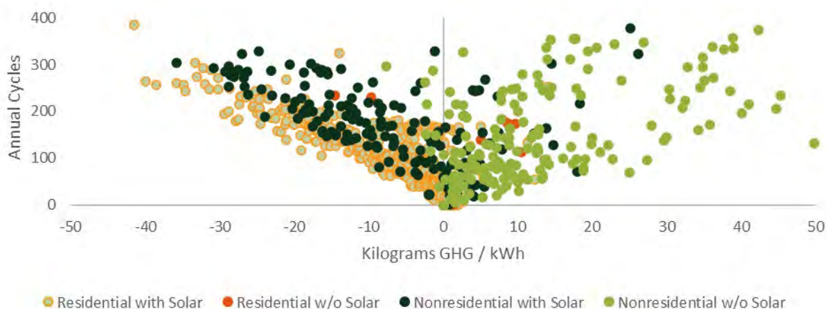
FIGURE 1-3: OBSERVED GHG EMISSIONS AND DISCHARGE FREQUENCY BY CUSTOMER SECTOR
