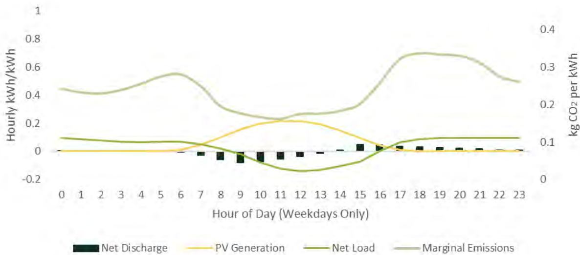
FIGURE 4-51: RESIDENTIAL DISCHARGE KWH PER CAPACITY KWH AND MARGINAL EMISSIONS FOR WINTER
