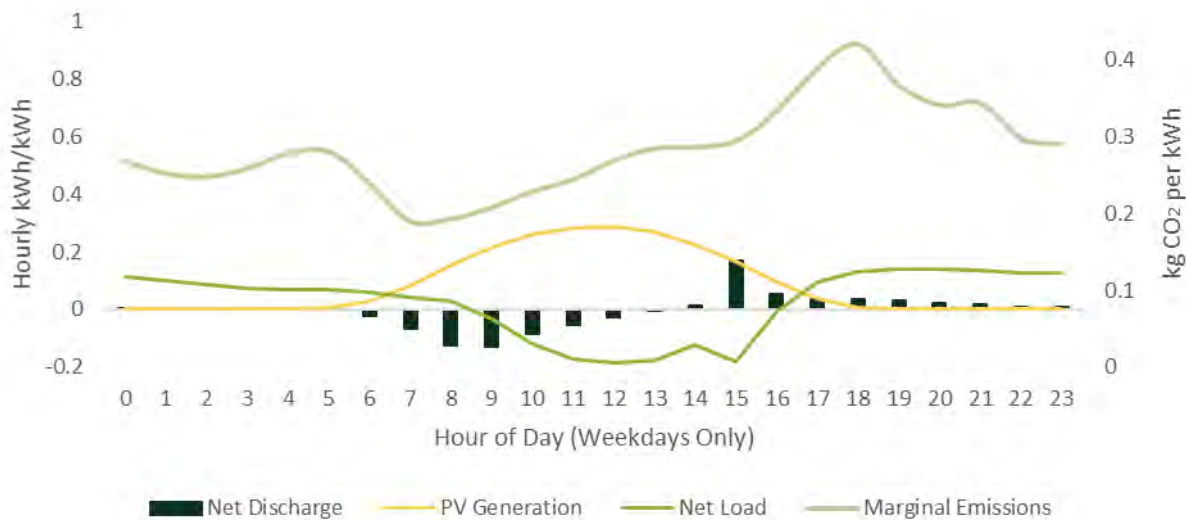
FIGURE 4-52: RESIDENTIAL DISCHARGE KWH PER CAPACITY KWH AND MARGINAL EMISSIONS FOR SUMMER
