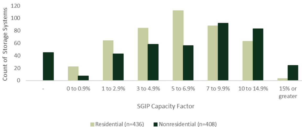
FIGURE 4-1: HISTOGRAM OF ANNUAL CAPACITY FACTOR BY CUSTOMER SECTOR
