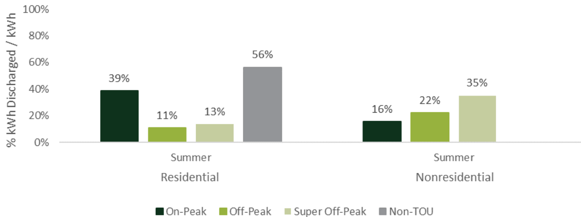
FIGURE 1-6: OBSERVED HOURLY NET DISCHARGE KWH PER CAPACITY KWH BY SUMMER TOU PERIOD
