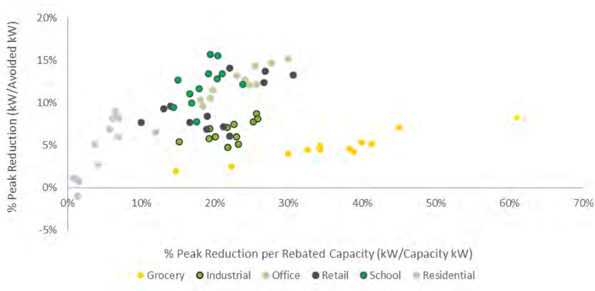
FIGURE 4-19: MONTHLY PEAK DEMAND REDUCTION (KW) PER AVOIDED PEAK (KW) BY CUSTOMER TYPE
