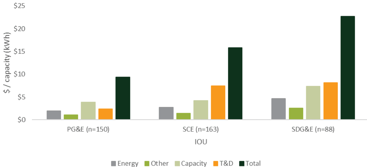
FIGURE 4-57: RESIDENTIAL MARGINAL AVOIDED COST $ PER CAPACITY KWH BY IOU
