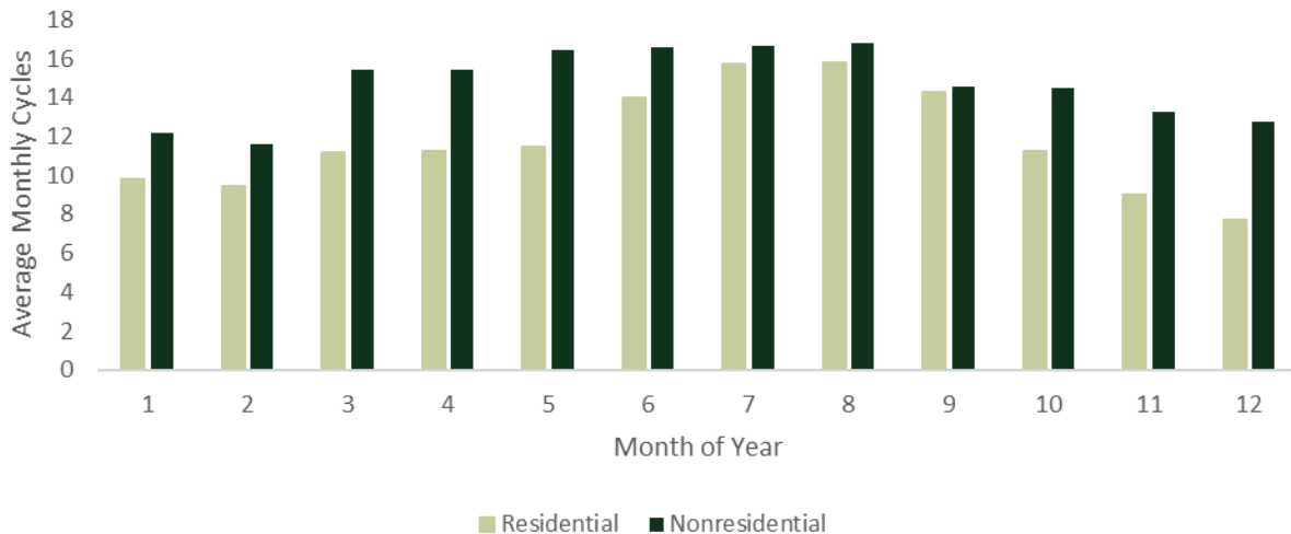
FIGURE 4-4: HISTOGRAM OF MONTHLY DISCHARGE CYCLES BY CUSTOMER SECTOR
