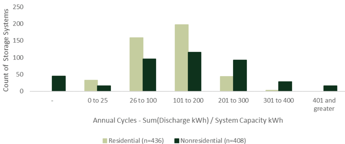
FIGURE 4-3: HISTOGRAM OF ANNUAL DISCHARGE CYCLES BY CUSTOMER SECTOR
