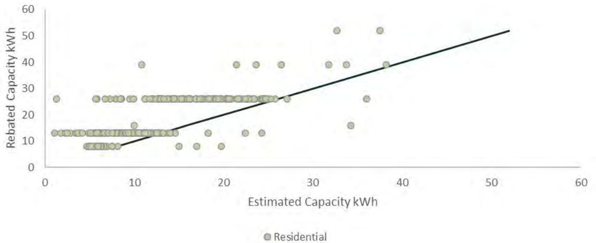
FIGURE 4-6: ESTIMATED CAPACITY KWH TO REBATED CAPACITY KWH FOR RESIDENTIAL SYSTEMS
