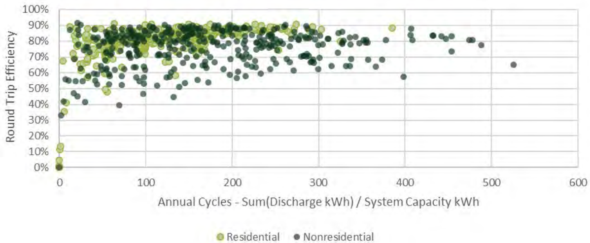
FIGURE 4-5: ANNUAL ROUNDTrip EFFICIENCY VERSUS ANNUAL DISCHARGE CYCLES
