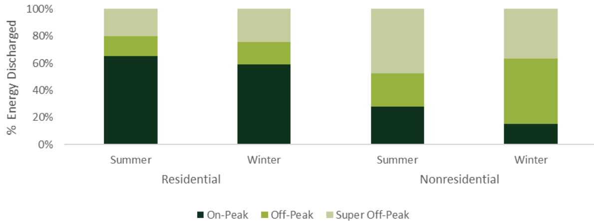
FIGURE 1-5: OBSERVED PERCENT DISCHARGE KWH BY TOU PERIOD AND CUSTOMER SECTOR
