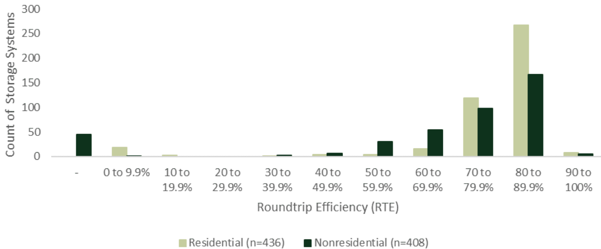
FIGURE 4-2: HISTOGRAM OF ANNUAL ROUNTRIP EFFICIENCY BY CUSTOMER SECTOR
