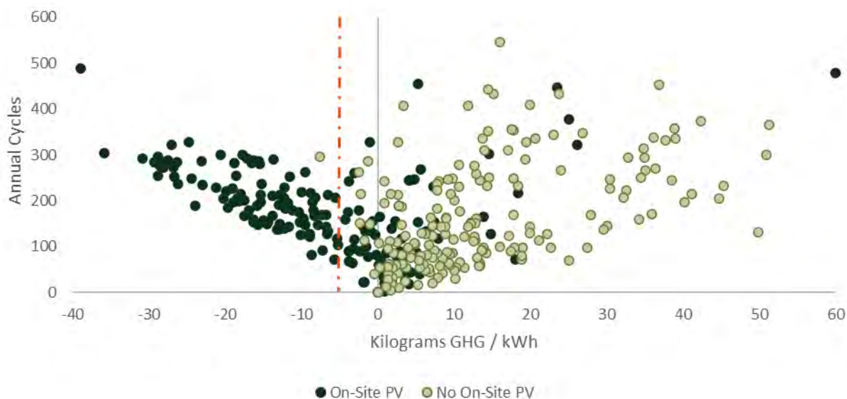
FIGURE 4-49: KILOGRAMS GHG / KWH INCREASE (+) DECREASE (-) FOR NONRESIDENTIAL SYSTEMS
