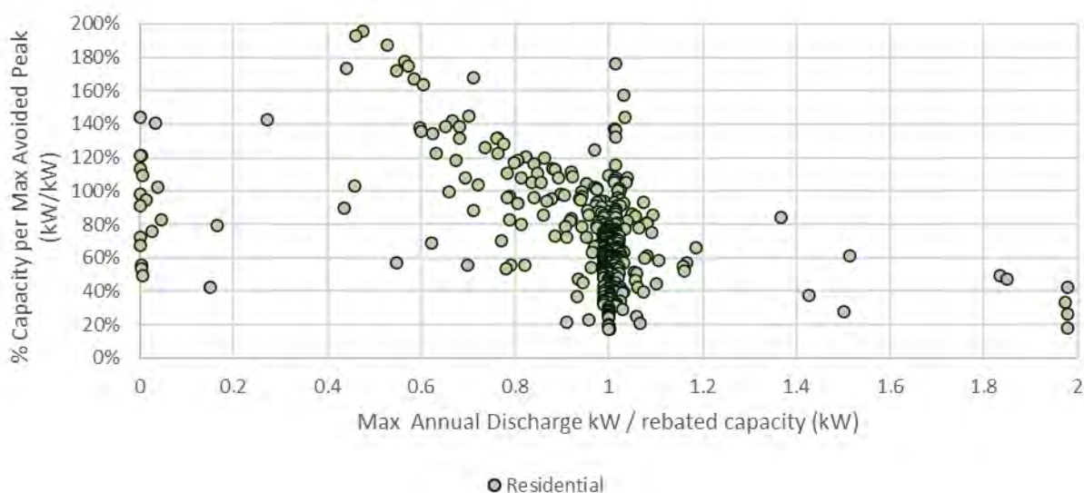
FIGURE 4-20: PERCENT CAPACITY (KW) PER MAX ANNUAL AVOIDED PEAK (KW) FOR RESIDENTIAL SYSTEMS
