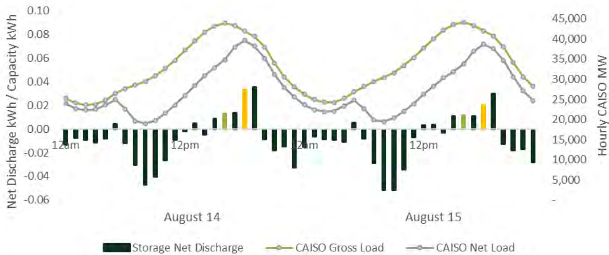
FIGURE 4-40: NONRESIDENTIAL HOURLY NET DISCHARGE DURING PEAK CAISO DAYS
