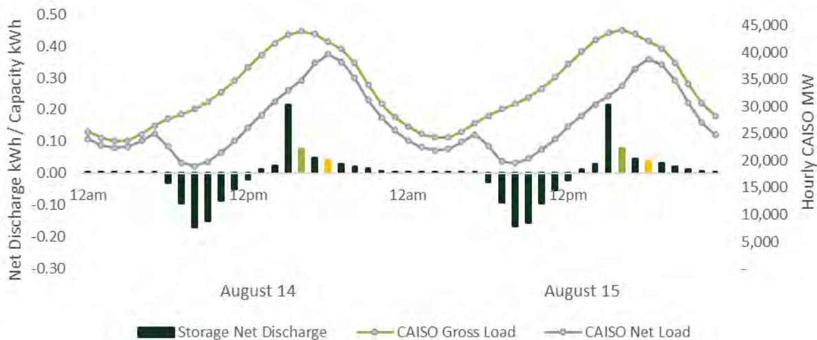
FIGURE 4-41: RESIDENTIAL HOURLY NET DISCHARGE DURING PEAK CAISO DAYS
