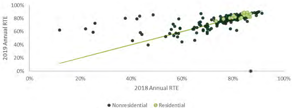
FIGURE 4-8: CROSS-YEAR ROUNDTRIP EFFICIENCY COMPARISON (2018 TO 2019)
