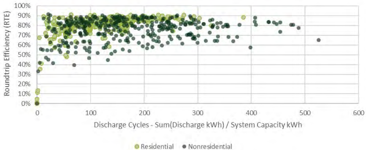
FIGURE 1-8: OBSERVED ROUNDTRIP EFFICIENCY VERSUS DISCHARGE FREQUENCY BY CUSTOMER SECTOR
