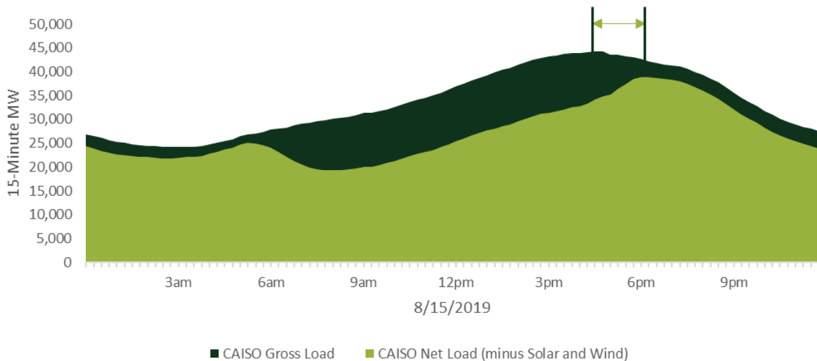
FIGURE 4-35: CAISO NET AND GROSS LOAD ON 8/15/2019 (TOP GROSS HOUR OCCURRED DURING 4 PM PST)
