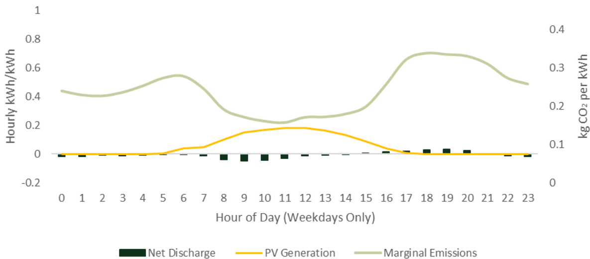
FIGURE 4-53: NONRESIDENTIAL DISCHARGE KWH PER CAPACITY KWH AND MARGINAL EMISSIONS FOR WINTER
