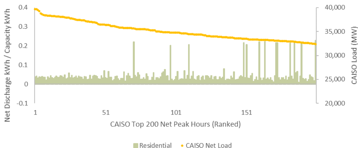
FIGURE 4-39: HOURLY NET DISCHARGE KWH PER KWH – CAISO TOP NET 200 HOURS FOR RESIDENTIAL
