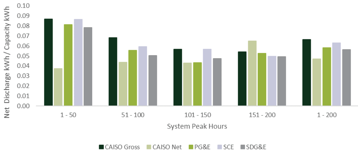
FIGURE 4-44: NET DISCHARGE KWH PER CAPACITY KWH DURING SYSTEM PEAK HOURS FOR RESIDENTIAL
