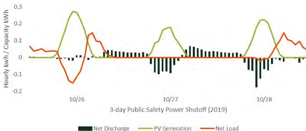
FIGURE 4-59: OBSERVED RESIDENTIAL STORAGE BEHAVIOR DURING PSPS EVENTS (WITH SOLAR PV)
