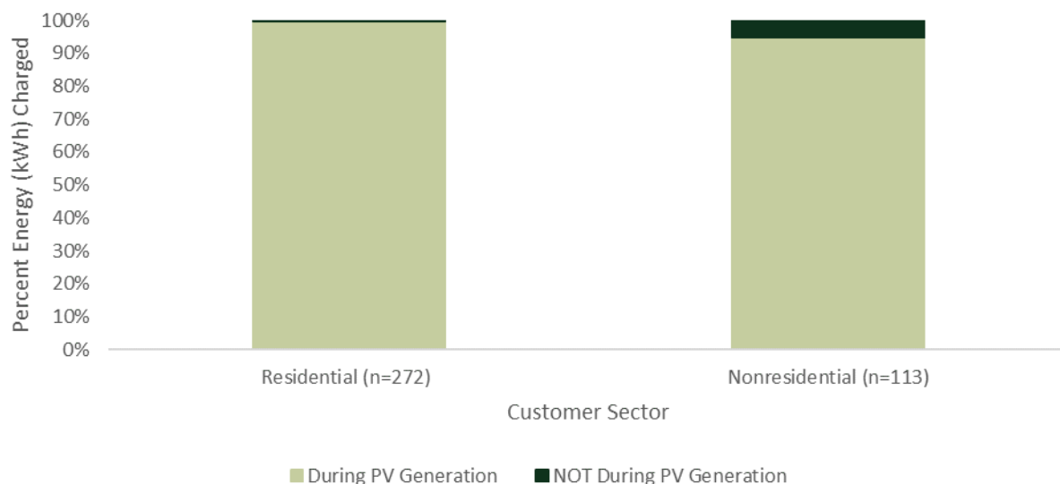
FIGURE 4-24: PERCENT CHARGE KWH DURING PV GENERATION BY CUSTOMER SECTOR
