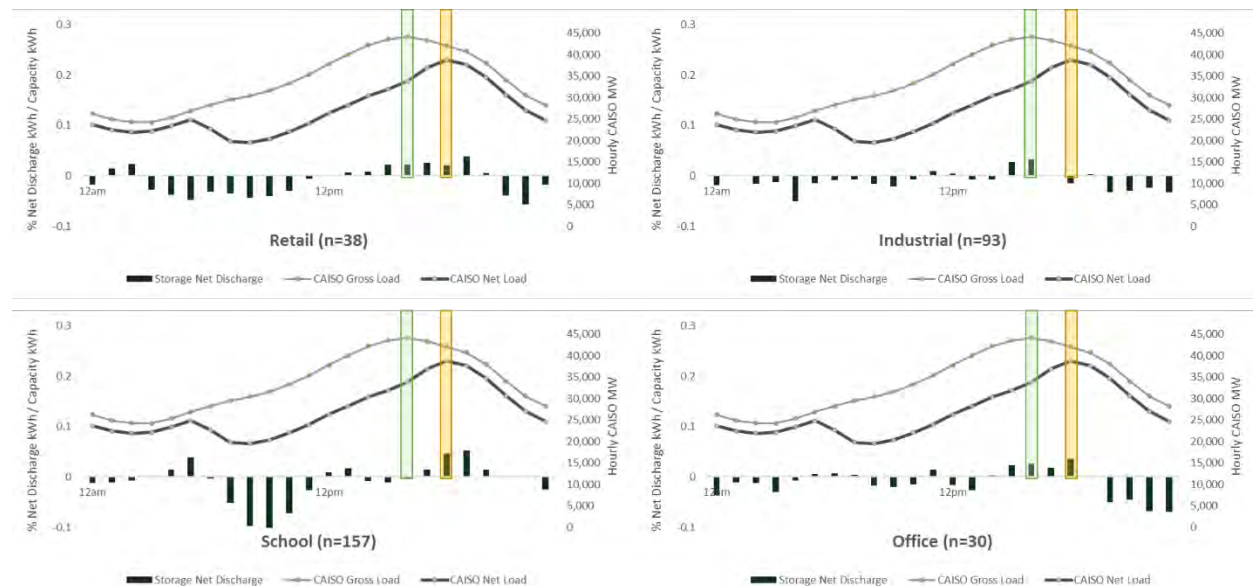
FIGURE 4-42: NONRESIDENTIAL HOURLY NET DISCHARGE DURING PEAK CAISO DAY BY FACILITY TYPE
