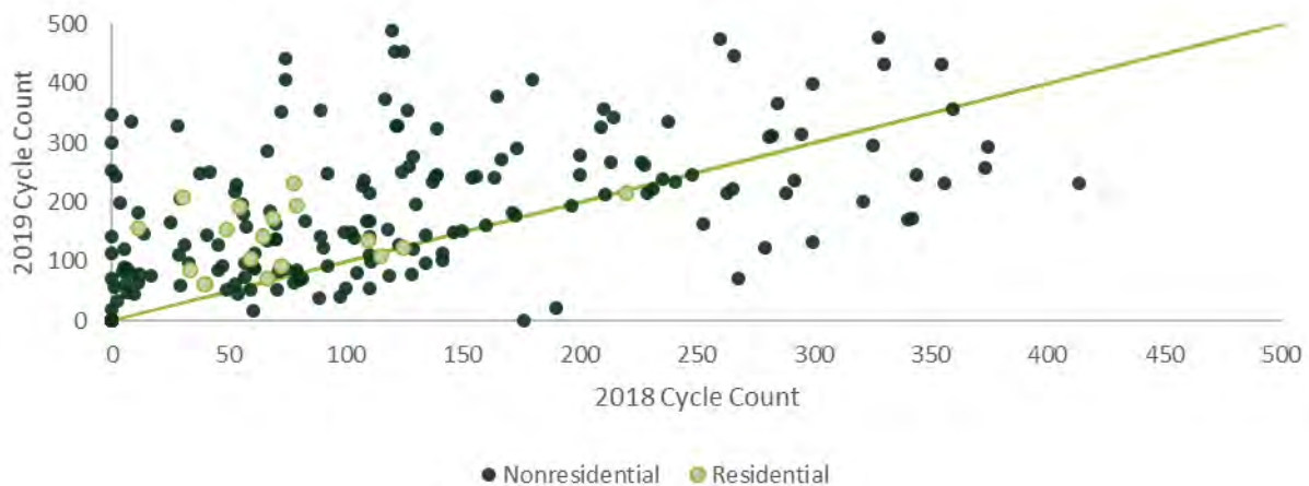
FIGURE 4-9: CROSS-YEAR DISCHARGE CYCLING COMPARISON (2018 TO 2019)
