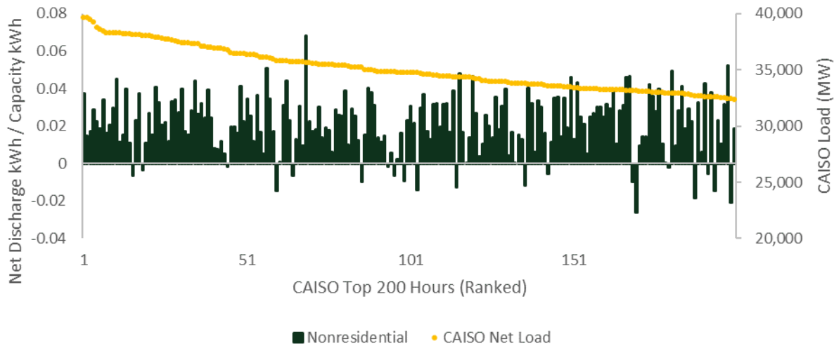
FIGURE 4-37: HOURLY NET DISCHARGE KWH PER KWH – CAISO TOP NET 200 HOURS FOR NONRESIDENTIAL
