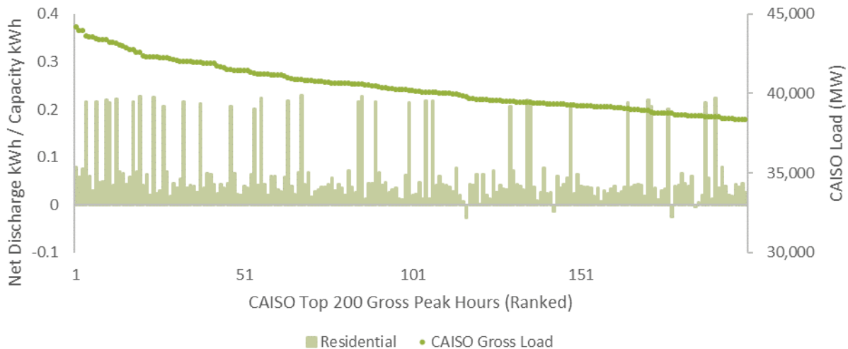
FIGURE 4-38: HOURLY NET DISCHARGE KWH PER KWH – CAISO TOP GROSS 200 HOURS FOR RESIDENTIAL
