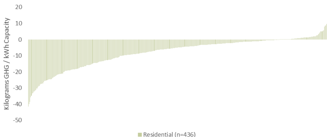
FIGURE 4-45: NET CO 2 EMISSIONS FOR RESIDENTIAL SYSTEMS (KILOGRAMS / KWH)
