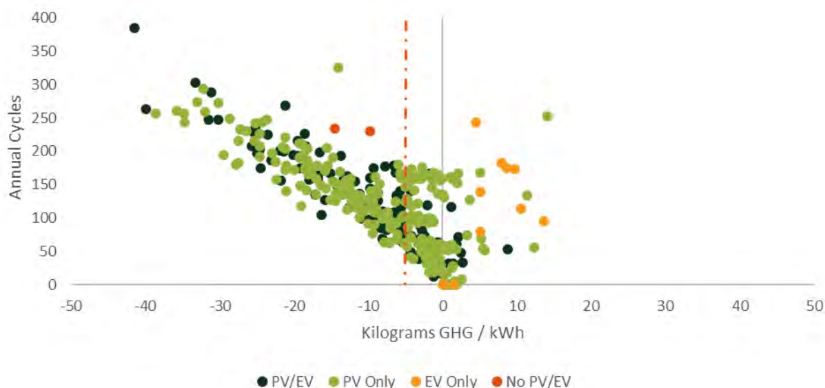
FIGURE 4-48: KILOGRAMS GHG / KWH INCREASE (+) DECREASE (-) FOR RESIDENTIAL SYSTEMS
