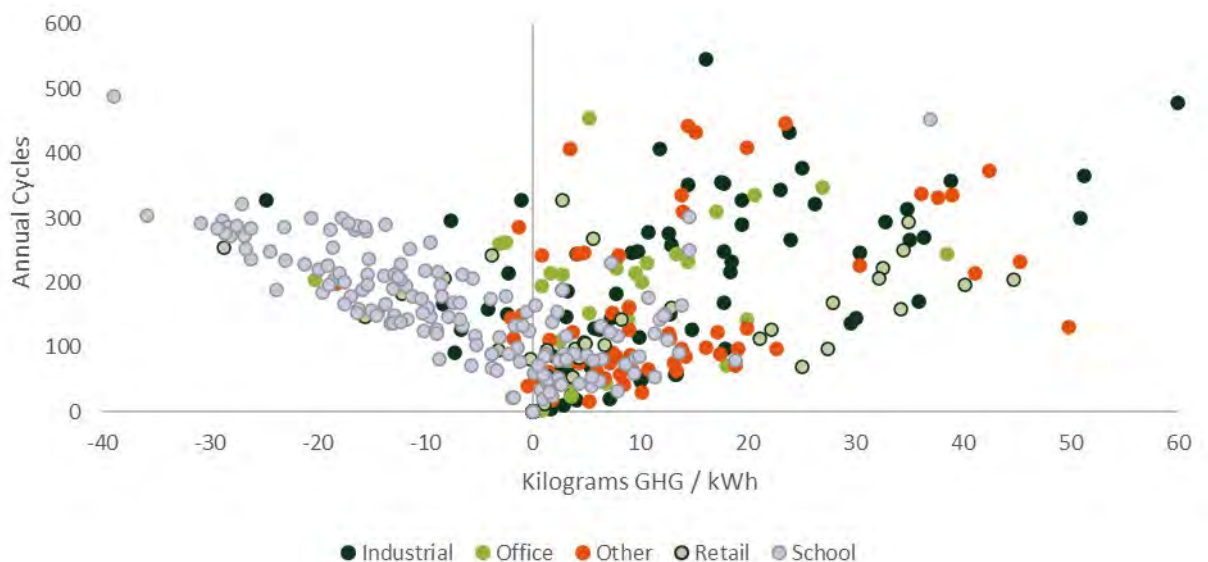
FIGURE 4-50: KILOGRAMS GHG / KWH INCREASE (+) DECREASE (-) FOR NONRESIDENTIAL SYSTEMS (BY FACILITY)
