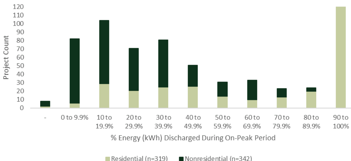
FIGURE 4-11: PERCENT KWH DISCHARGE DURING PEAK PERIOD BY CUSTOMER SECTOR
